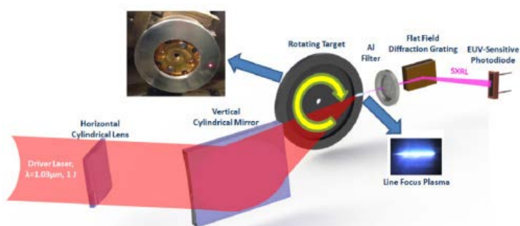
Figure 1: Schematic of table-top EUV laser. An optical laser beam is focused into a selected solid rotating target to generate a line focus plasma from which an EUV laser beam is generated.
